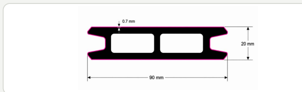
CROSS-SECTION
