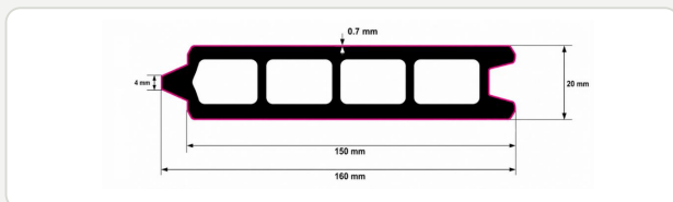
CROSS-SECTION
