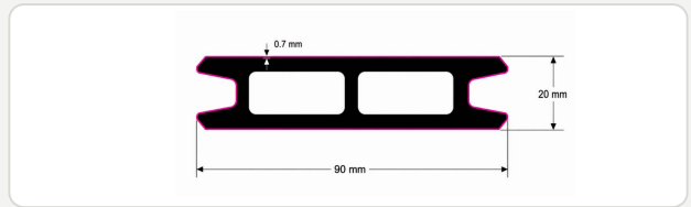
CROSS-SECTION
