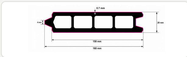
CROSS-SECTION
