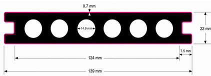
CROSS-SECTION
