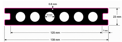
CROSS-SECTION
